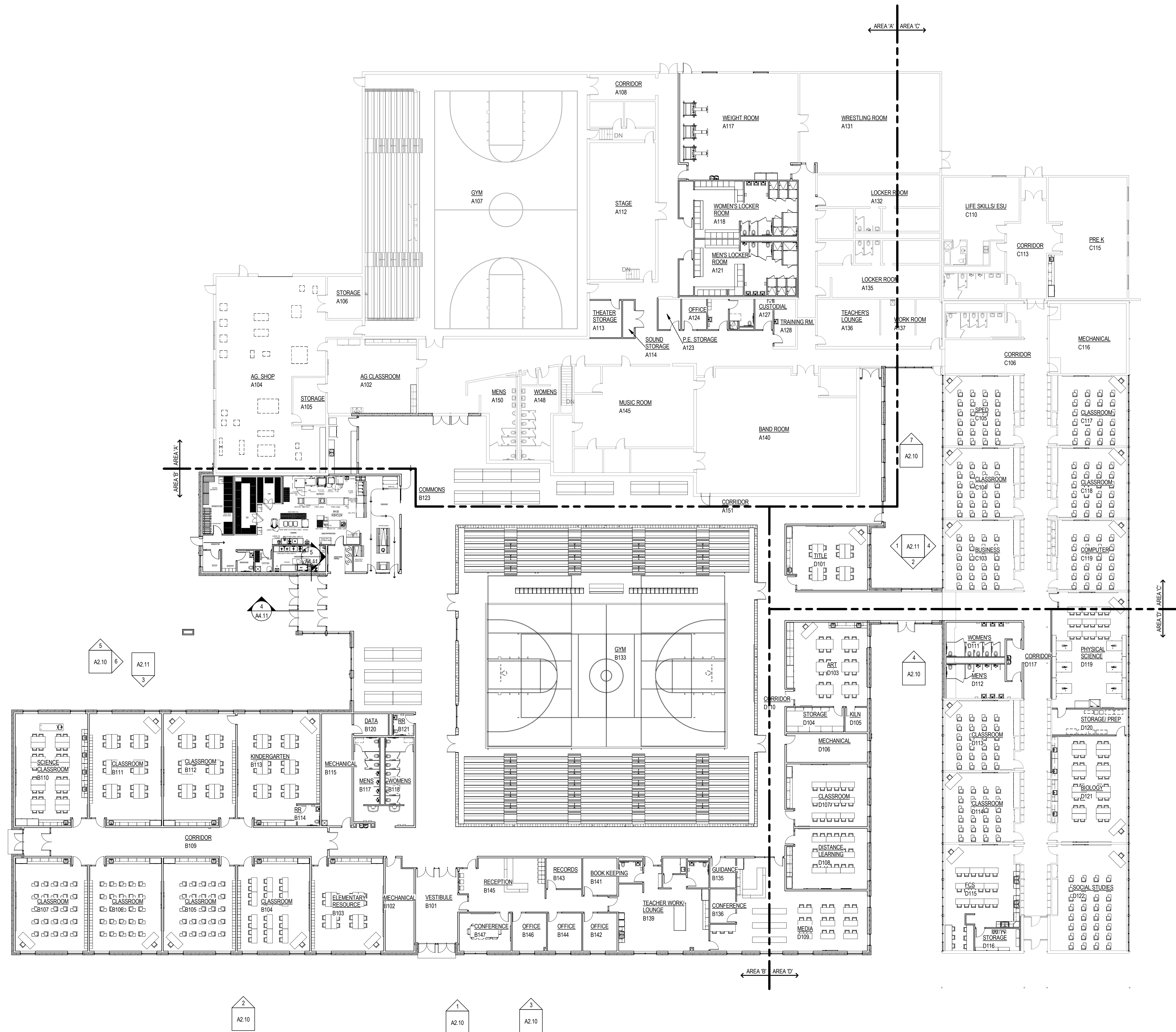
1 FIRST FLOOR ORIENTATION PLAN SCALE: 1/16" = 1'-0"
